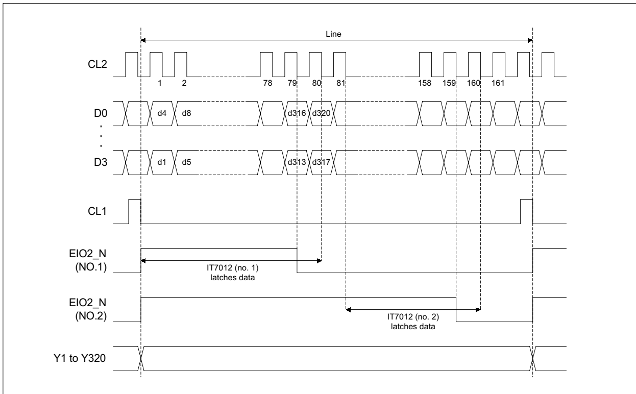
Figure 6-2. Data Latch Timing (1)
