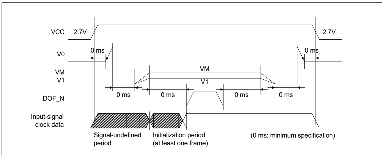
Figure 7-1. IT7012C/H Power On/Off Scenario
