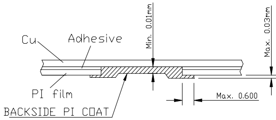
Detail of flex
