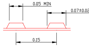
CROSS SECTION OF OUTPUT LEADS
