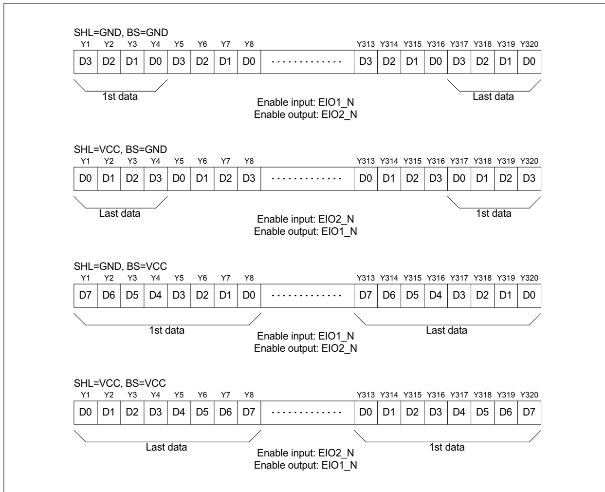
Figure 6-1. Data Output Destination
