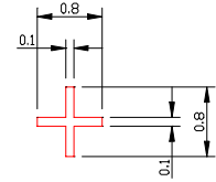
GOOD DEVICE HOLE
