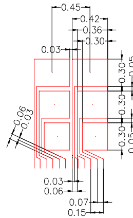
DETAIL : C (Output Side TEST PADS)
