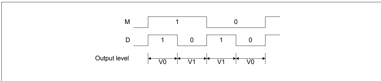
Figure 5-2. Selection of LCD Drive Output Level
