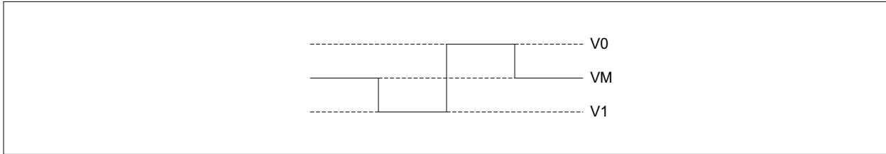
Figure 5-1. LCD Drive Level Voltage
