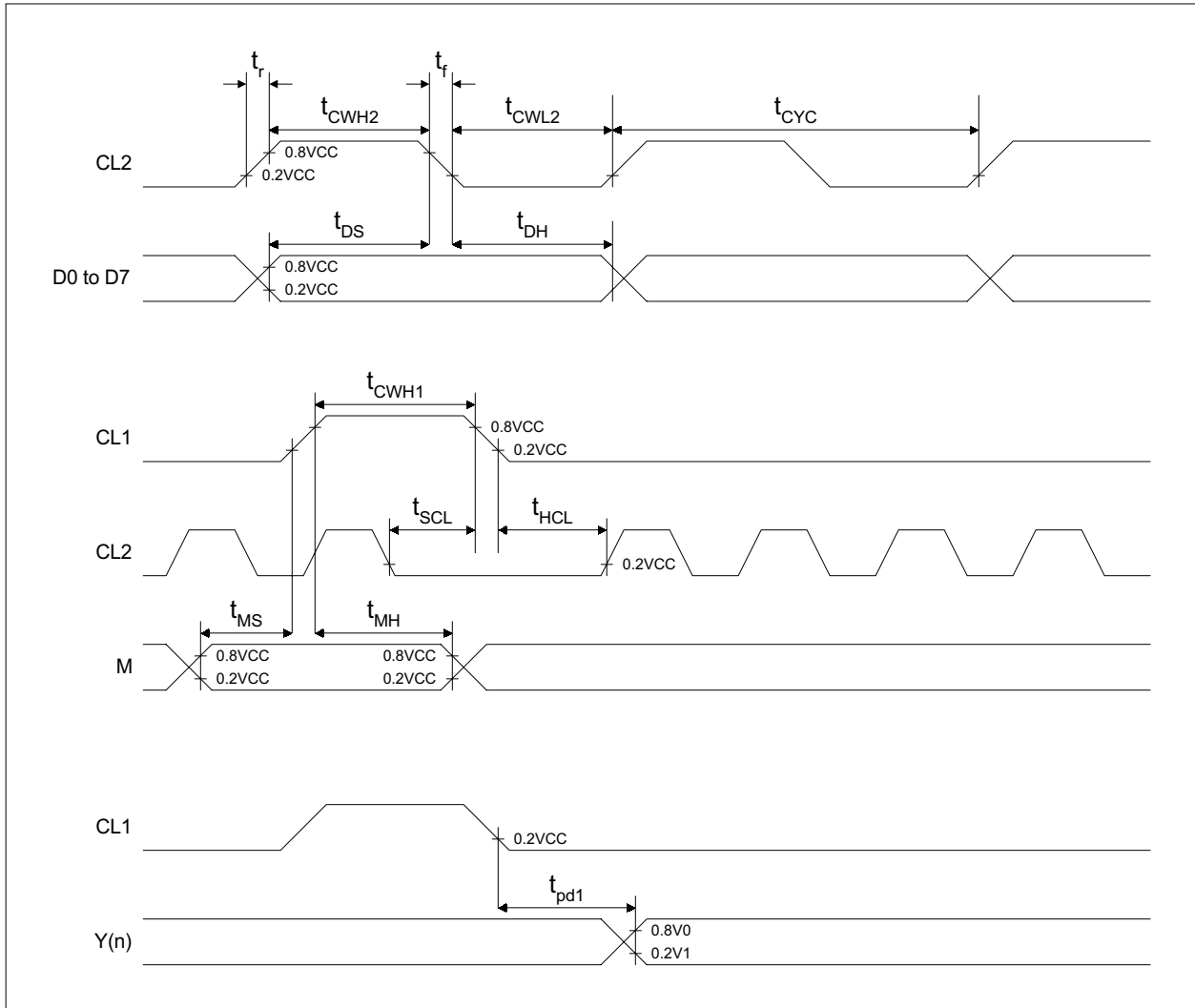
Figure 8-2. AC Characteristics
