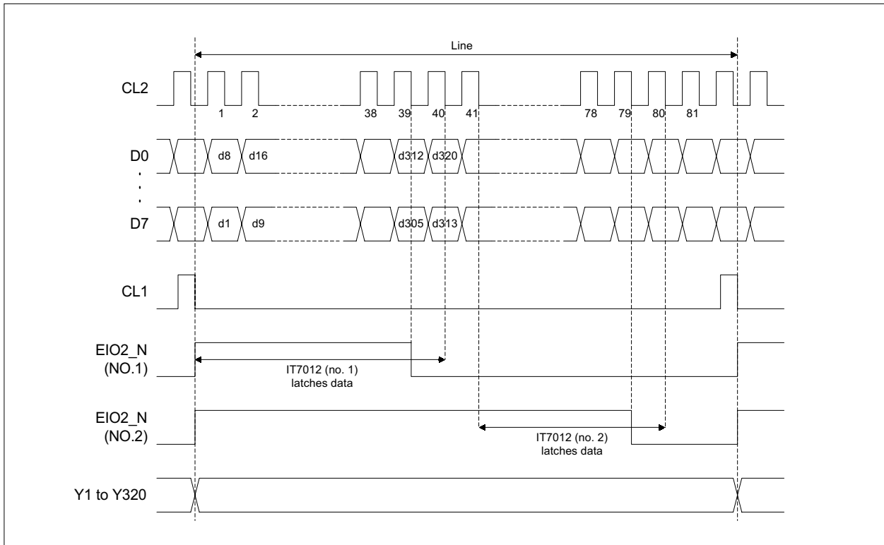
Figure 6-3. Data Latch Timing (2)
