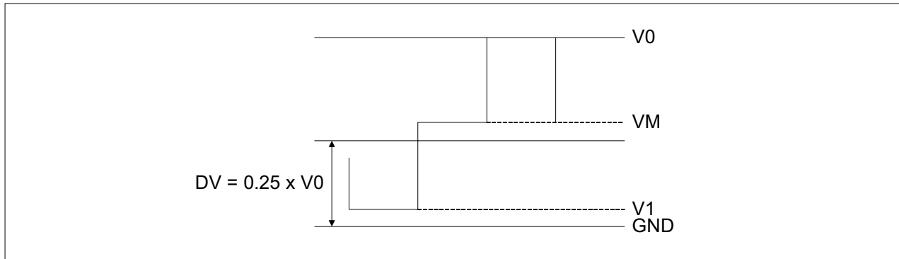
Figure 7-2. Relationship Between Driver-Output Waveforms and Each Level Voltage
