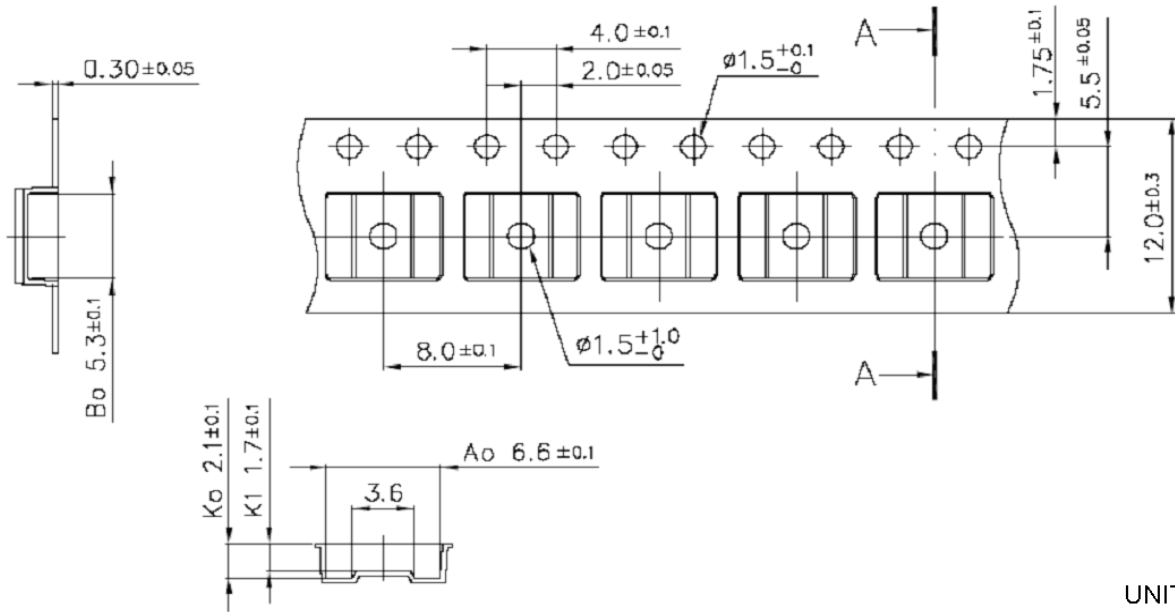
Carrier Tape
