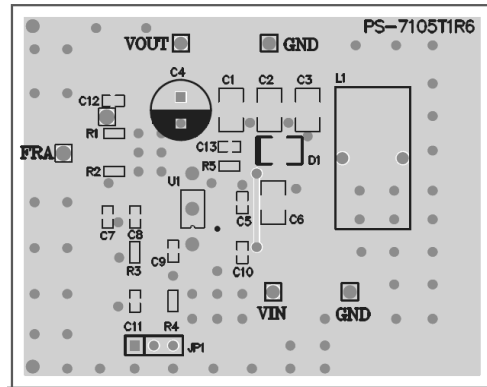
Bottom Layer (Top view)
