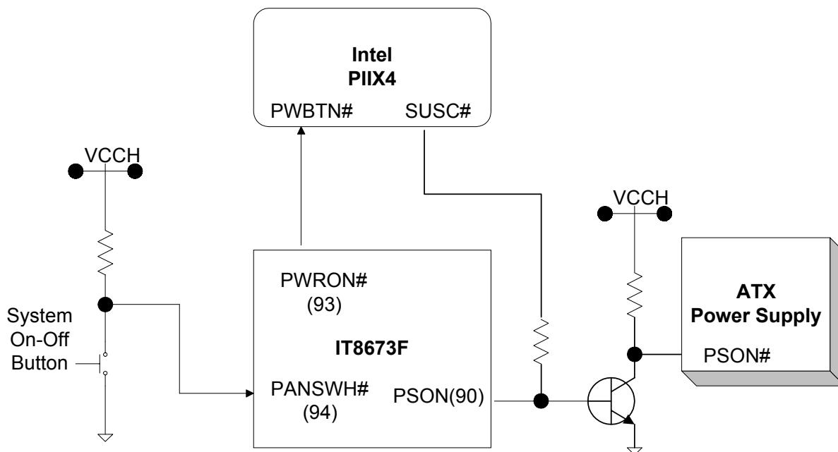
Figure 7-1. IT8673F Special Applications Circuitry for Intel PIIX4
