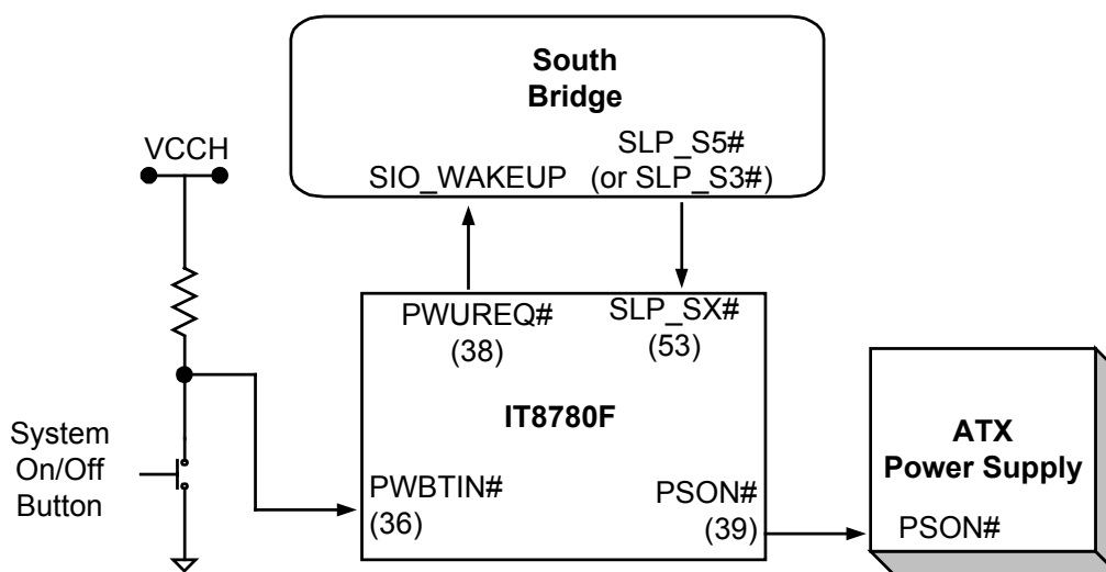
Figure 7-1. IT8780F Power Control Suggestion Applications Circuitry
