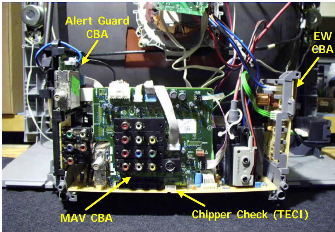
Chassis Layout
