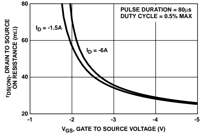
FIGURE 8. DRAIN TO SOURCE ON RESISTANCE vs GATE VOLTAGE AND DRAIN CURRENT
