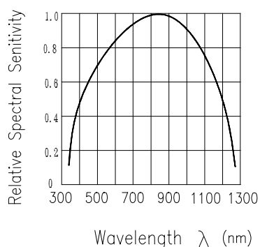
Fig.5 Spectral Sensitivity
