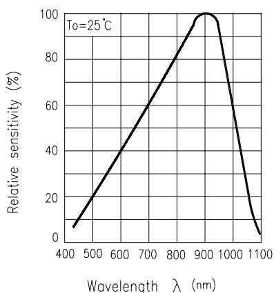
Fig.3 Spectral Sensitivity
