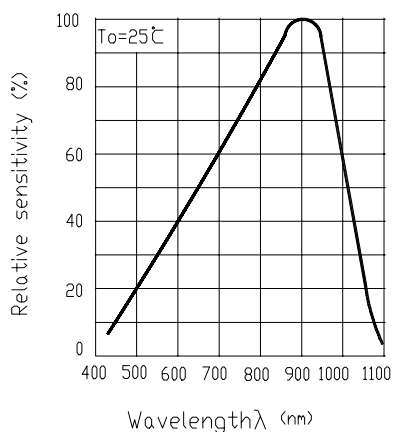
Fig.3 Spectral Sensitivity
