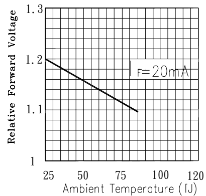
Fig. 6 Forward Voltage vs. Ambient Temperature (°C)
