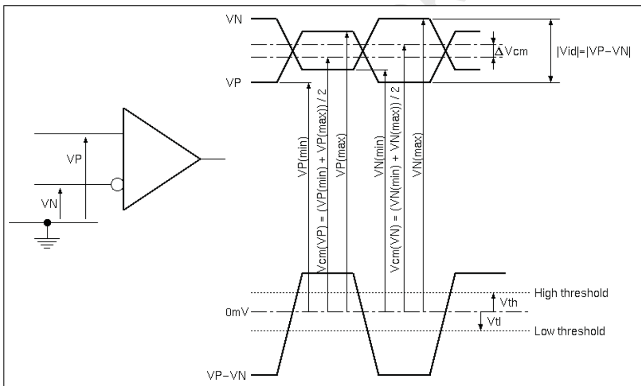
Figure. Voltage Definitions
