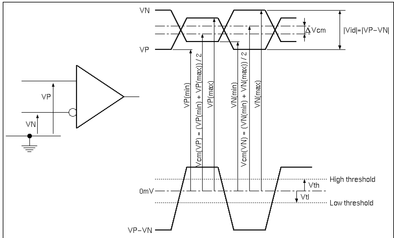
Figure. Voltage Definitions
