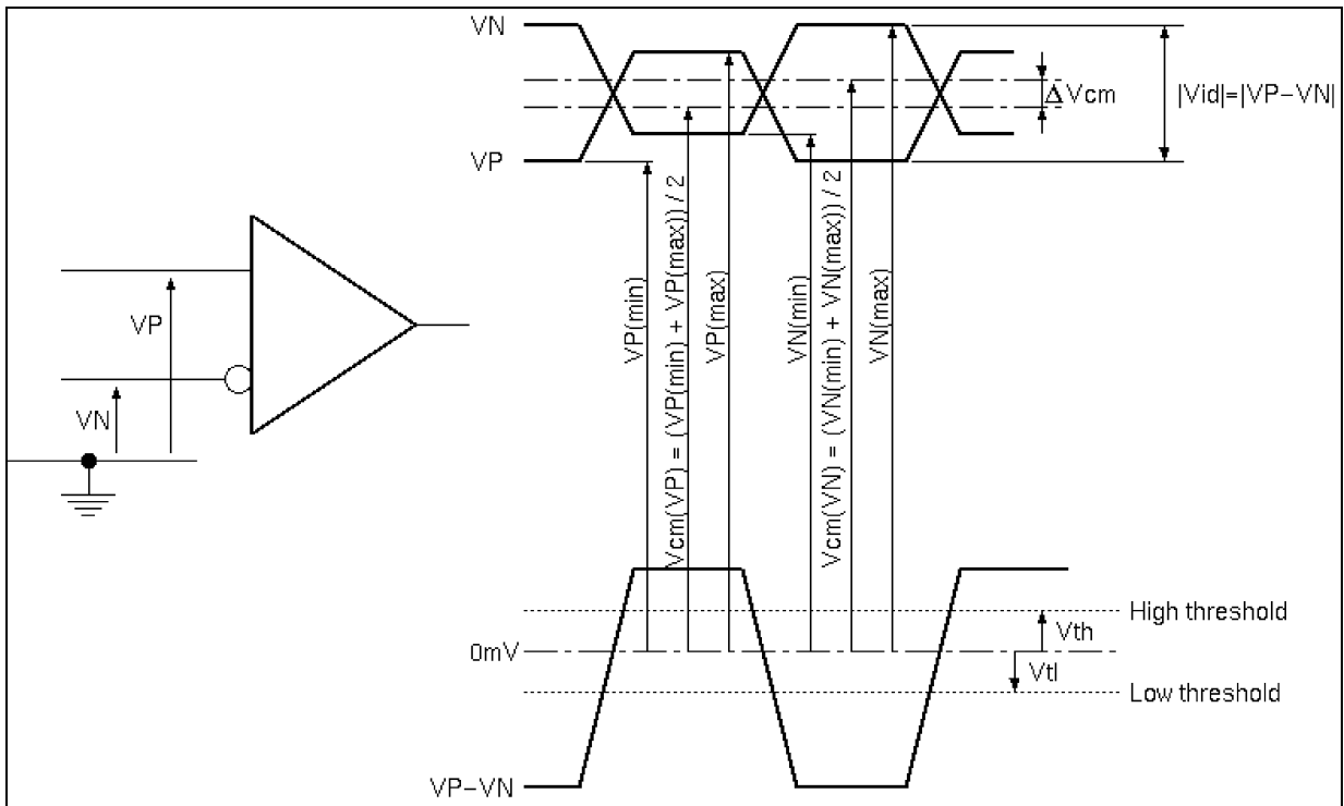
Voltage Definitions
