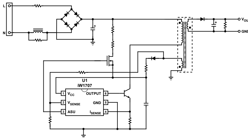
Figure 3.1: iW1707 Typical Application Circuit
