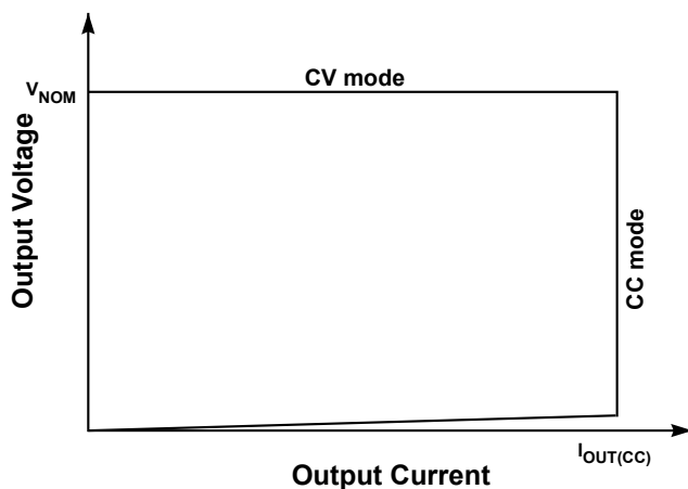
Figure 9.4: Power Envelope
