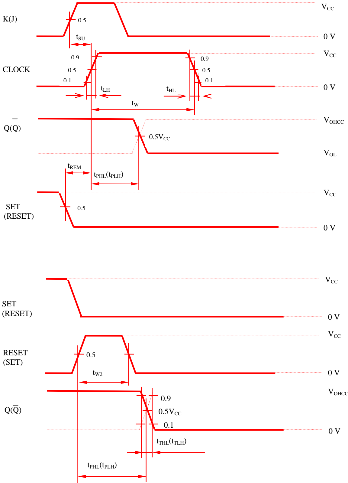
Figure 1. Switching Waveforms
