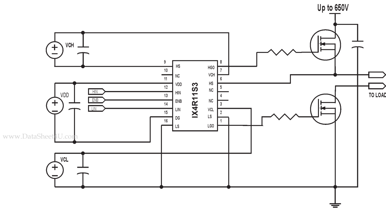
Figure 1. Typical Circuit Connection
