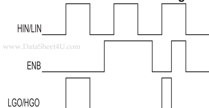
Figure 3. INPUT/OUTPUT Timing Diagram
