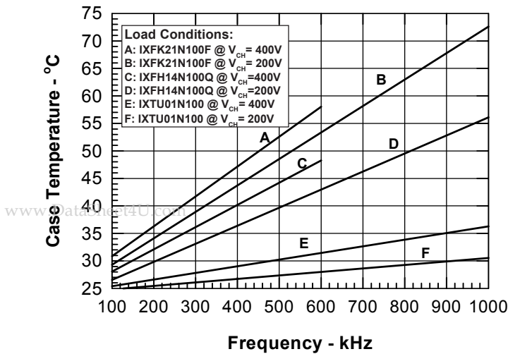
Fig. 24a. Case temperature rise vs. switching frequency for IX6R11S6
