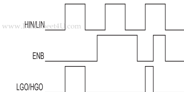
Figure 3. INPUT/OUTPUT Timing Diagram
