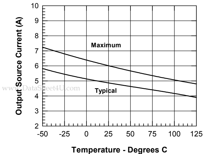
Fig. 17a. Output source current vs. temperature
