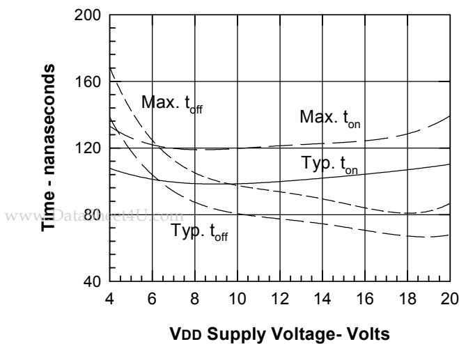
Fig. 10a. Low side turn-on and turn-off delay times vs. V_{DD} supply voltage.
