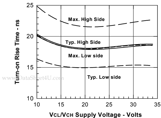
Fig. 12b. Turn-on rise times vs. bias supply voltages.
