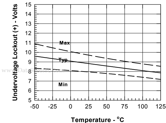
Fig. 20a. V_{CL} Undervoltage positive trip vs. temperature.
