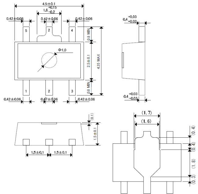
SOT-89-5, Units: mm
