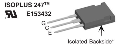
G = Gate C = Collector E = Emitter
