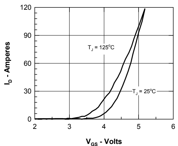
Figure 6. Admittance Curves
