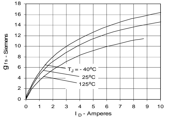
Fig. 9. Transconductance
