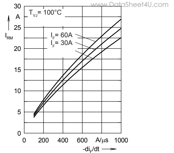
Fig. 19. Peak reverse current I_{RM}
