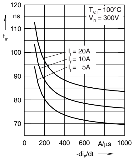
Fig. 17. Recovery time t_{rr} versus -di_F/dt
