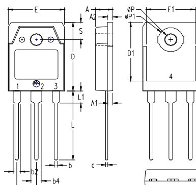
TO-3P (IXGQ) Outline
