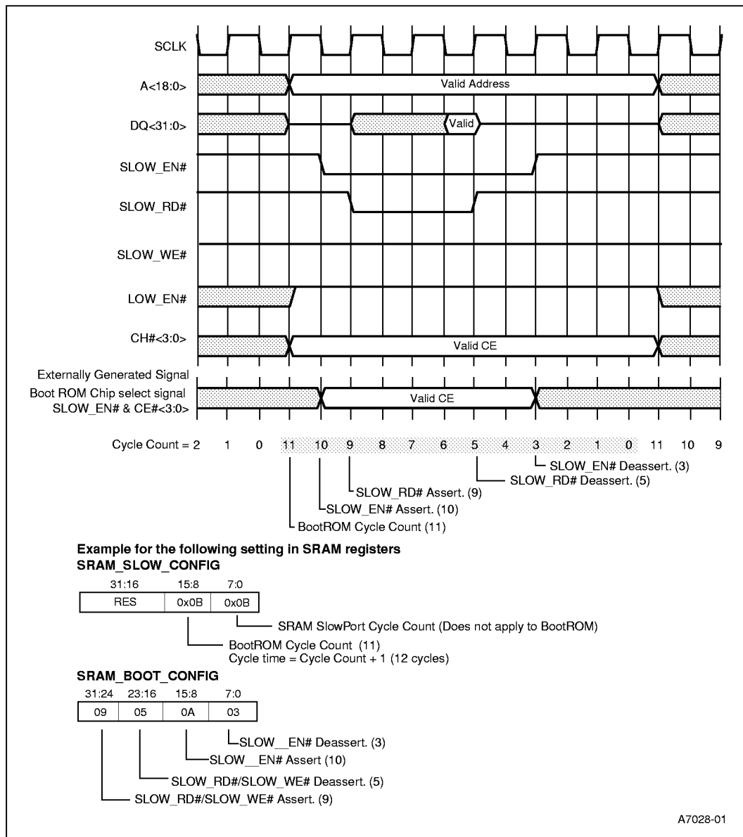
Figure 52: BootROM Read
