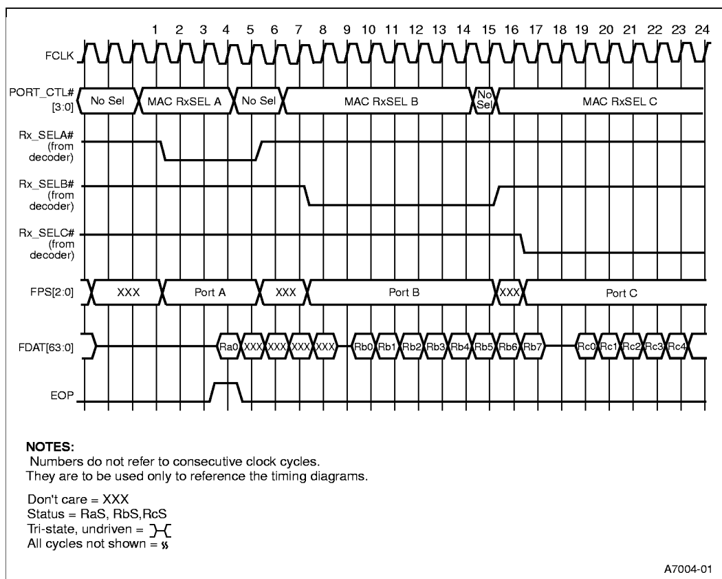
Figure 17: 64-Bit Bidirectional IX Bus Timing - Consecutive Receives with EOP on 1st Data Return, No Status Transfer
