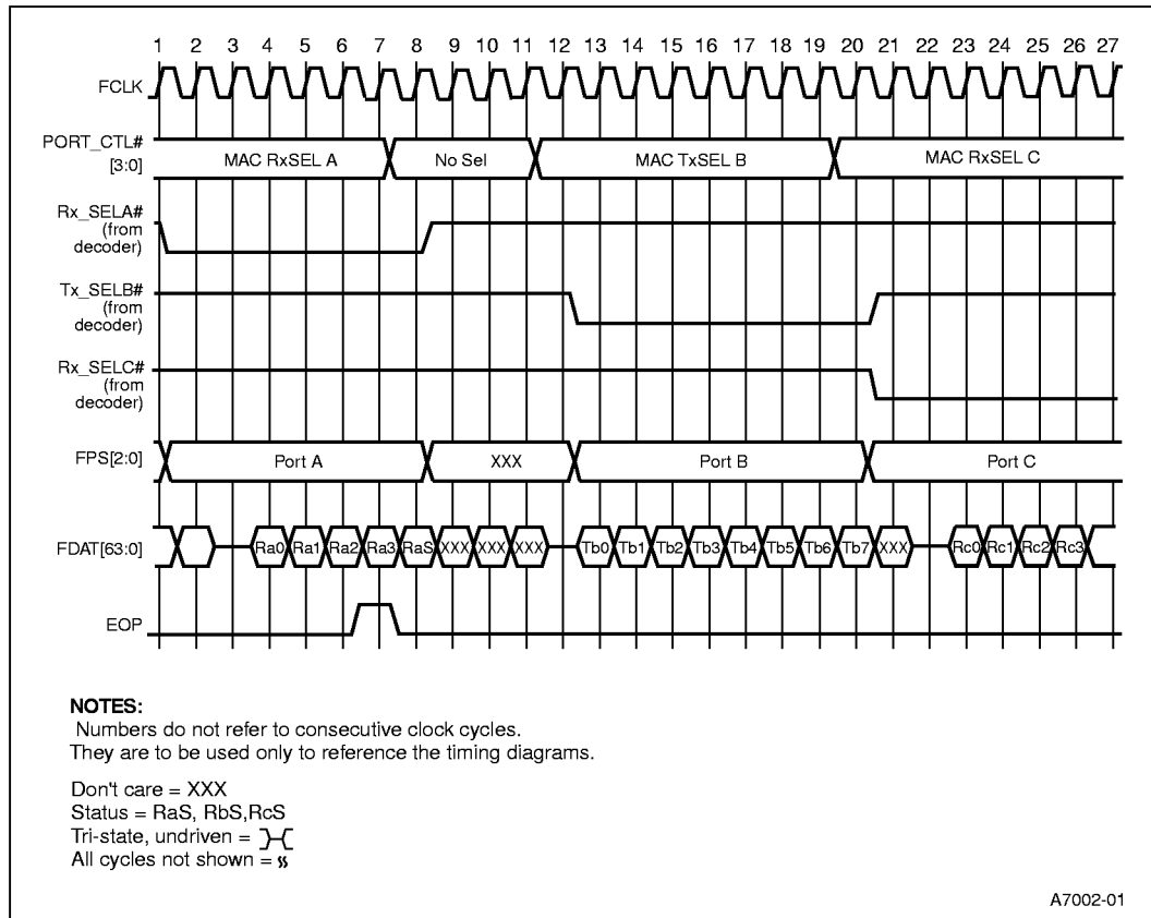
Figure 24: 64-Bit Bidirectional IX Bus Timing - Consecutive Receive and Transmit with EOP on 4th Data Return
