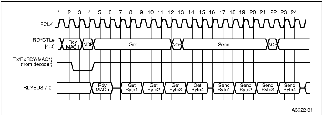
Figure 42: Ready Bus Control Timing, Fetch Ready Flags - Flow Control - Fetch Ready Flags, 1-2 MACs (with No External Registered Decoder) - RDYBUS_TEMPLATE_CTL[10]=1
