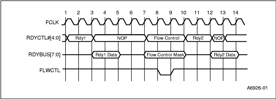
Figure 43: Ready Bus Control Timing, Fetch Ready Flags - Flow Control - Fetch Ready Flags, 1-2 MACs (with No External Registered Decoder) - RDYBUS_TEMPLATE_CTL[10]=0
