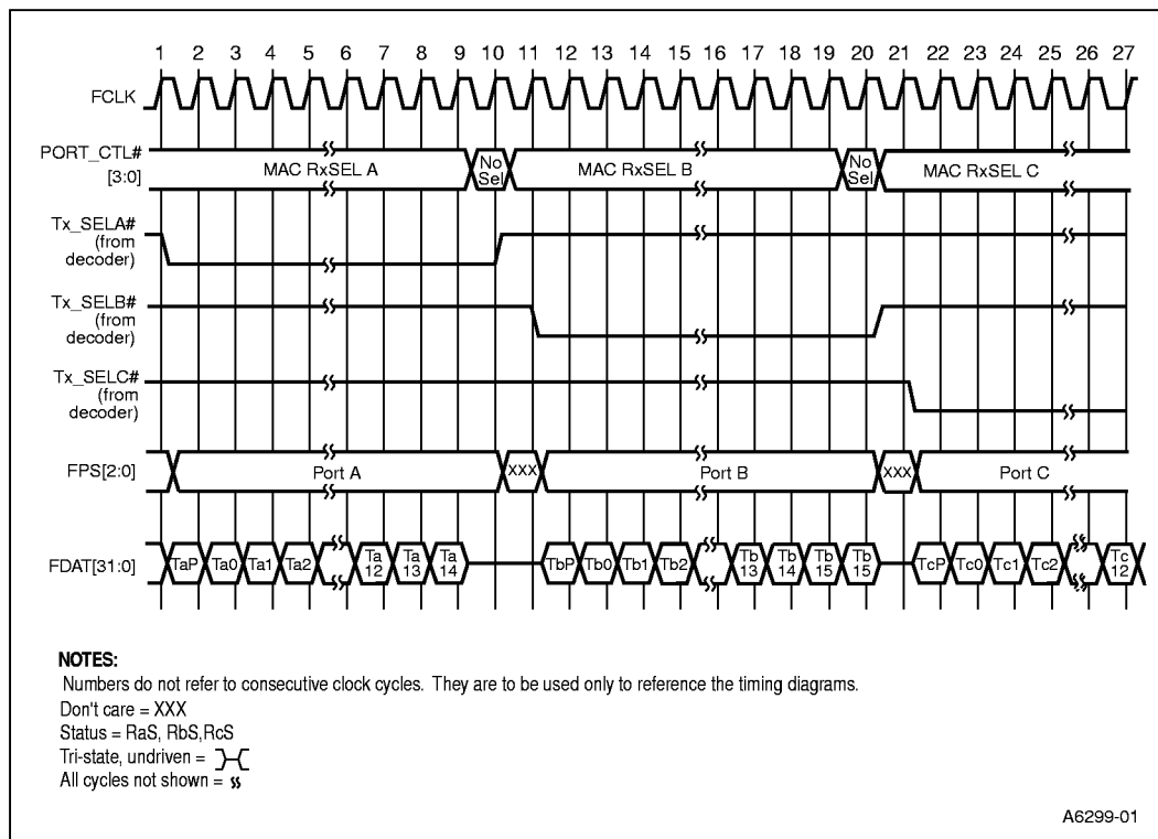
Figure 37: 32-Bit Unidirectional IX Bus Timing - Consecutive Transmits with Prepend
