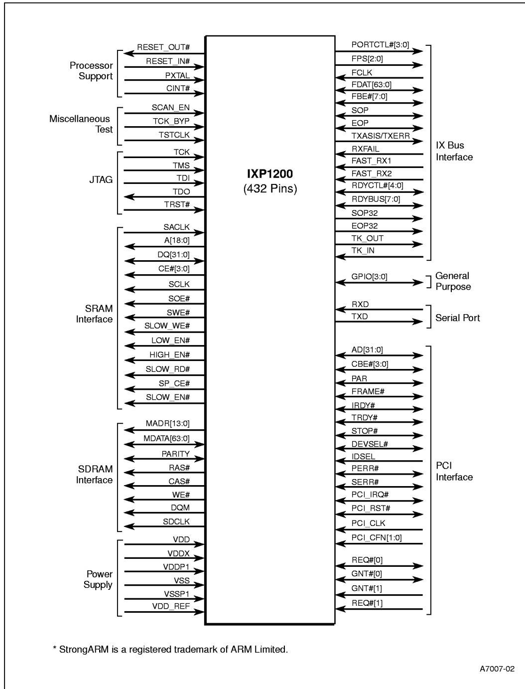
Figure 6: Pinout Diagram
