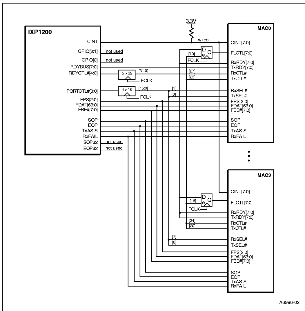
Figure 8: 64-Bit Bidirectional IX Bus, 3+ MAC Mode
