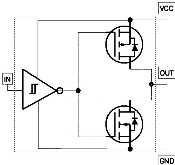
Fig. 1 Block Diagram and Truth Table per Driver
