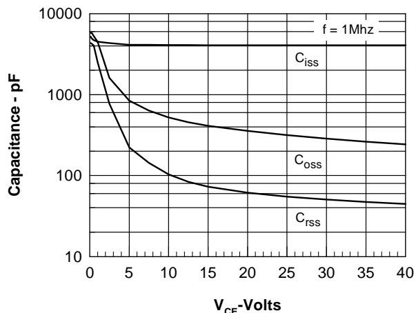
Figure 6. Capacitance Curves
