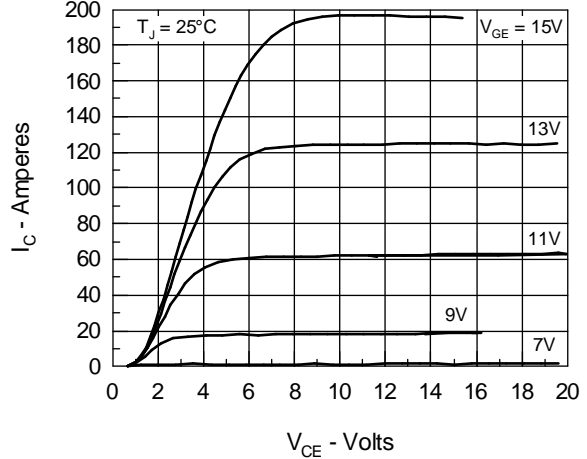
Fig. 2 Output Characteristics
