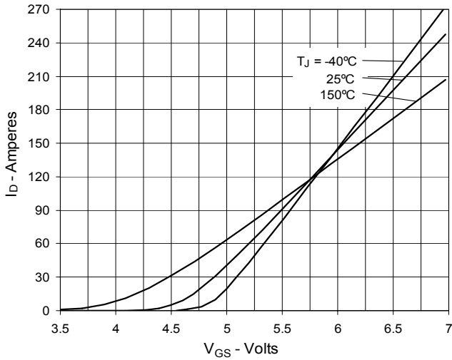
Fig. 7. Input Admittance
