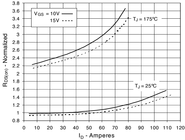
Fig. 5. R_{DS(on)} Normalized to I_D = 25A Value vs. Drain Current
