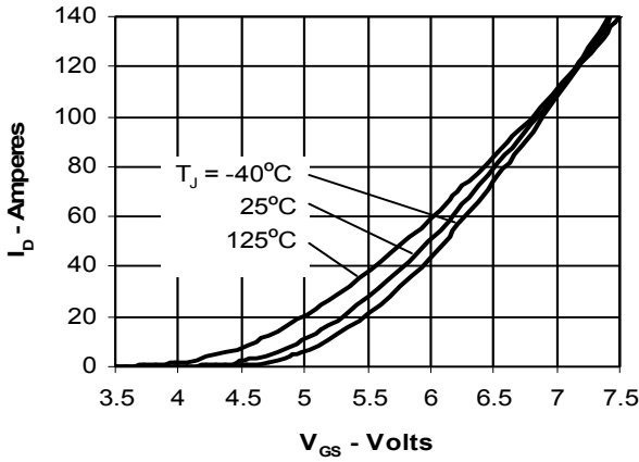
Fig. 7. Input Admittance
