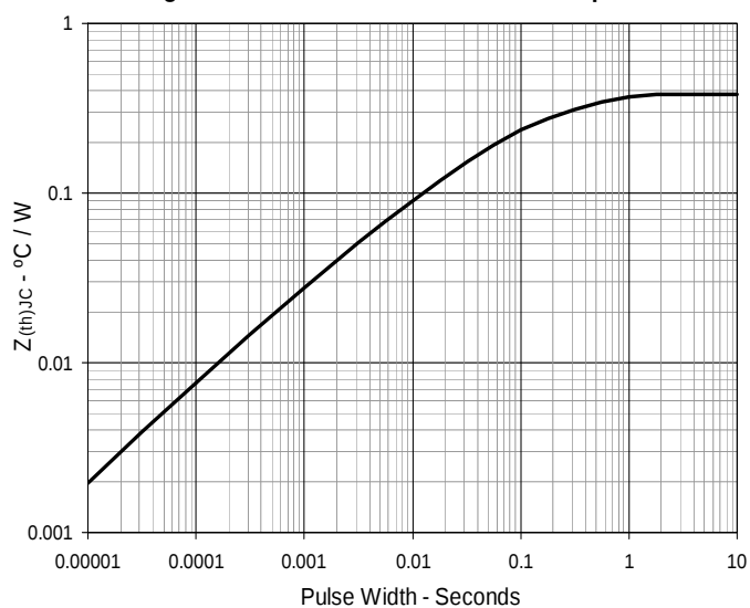
Fig. 14. Maximum Transient Thermal Impedance
