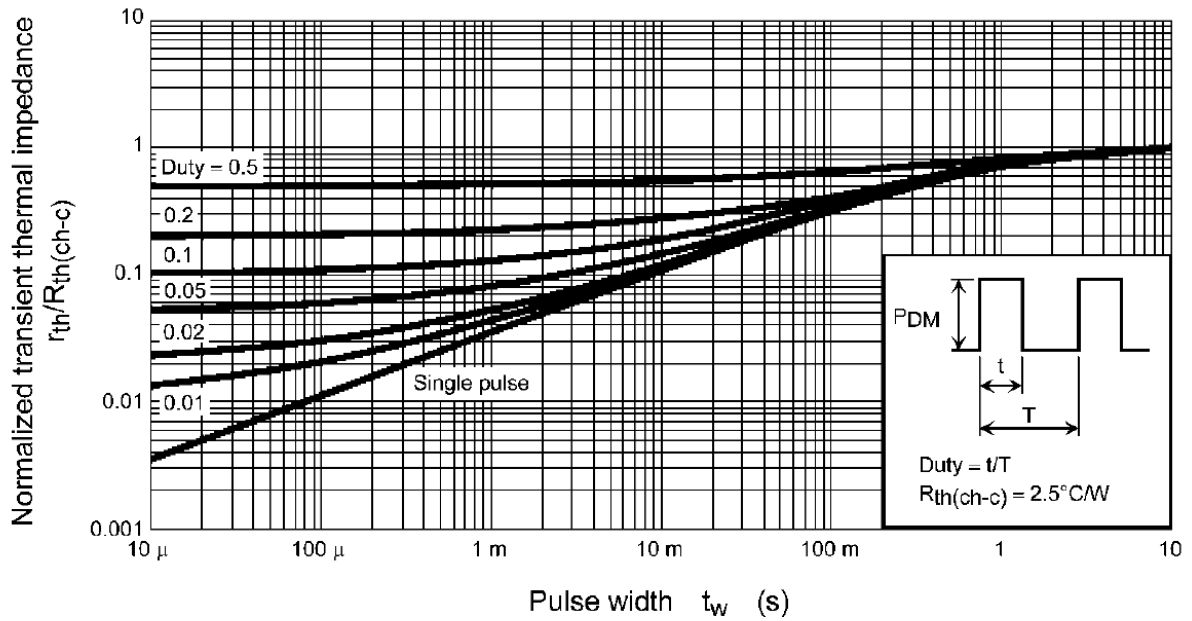
Transient Thermal Response Curve JCS10N80GDC
