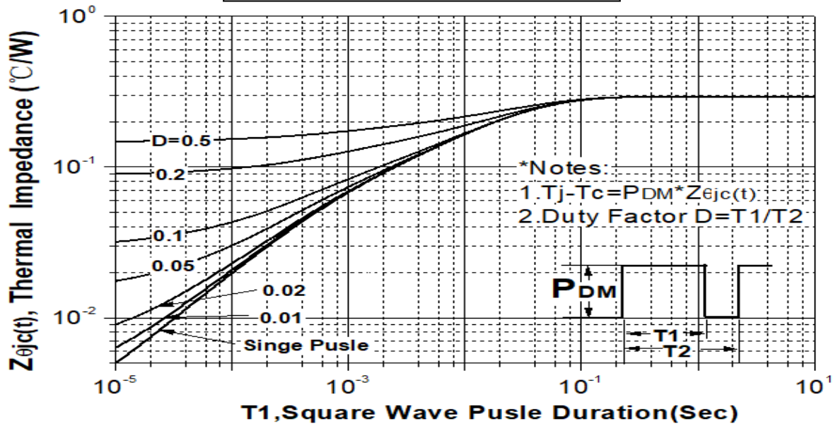
Transient Thermal Response Curve JCS10N80GDC
