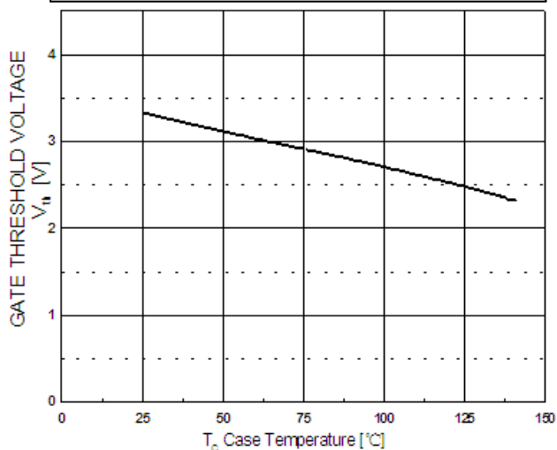
V TH vs. Case Temperature
