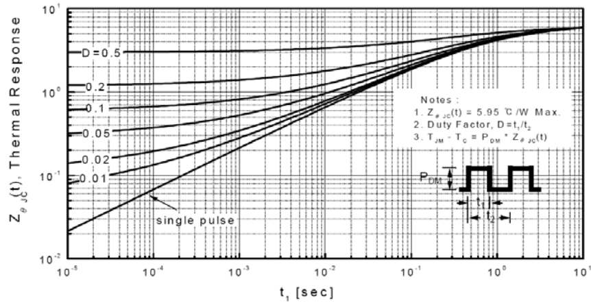
Transient Thermal Response Curve For JCS1N60F
