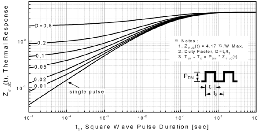
Transient Thermal Response Curve For JCS1N60V/R
