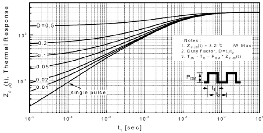
Transient Thermal Response Curve For JCS1N60S/B/C
