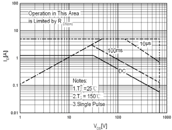
Maximum Safe Operating Area For JCS1N60F
