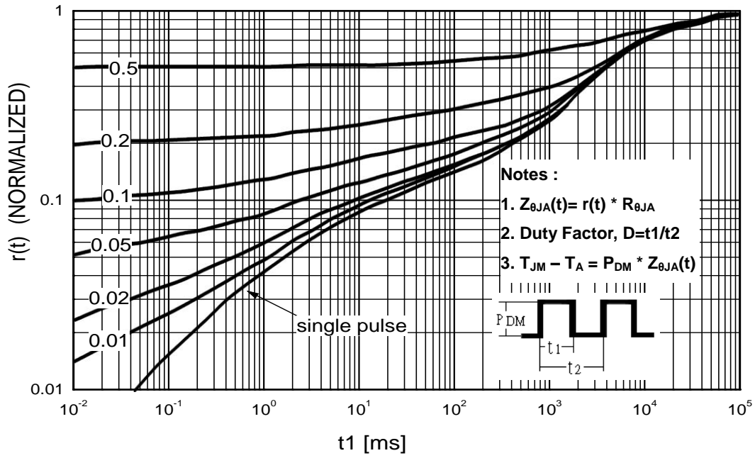
Transient Thermal Response Curve For JCS2N60TC
