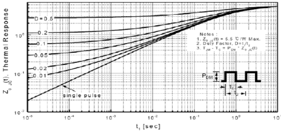
Transient Thermal Response Curve For JCS2N65F
