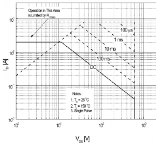
Maximum Safe Operating Area For JCS2N65F
