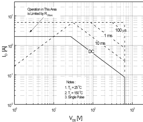
Maximum Safe Operating Area For JCS2N65TC
