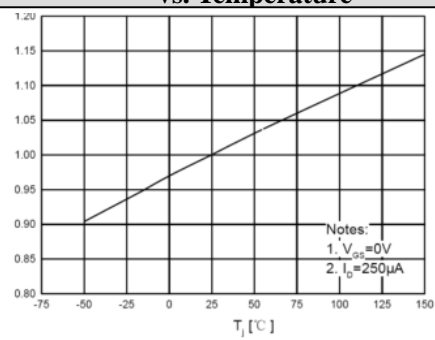
Breakdown Voltage Variation vs. Temperature
