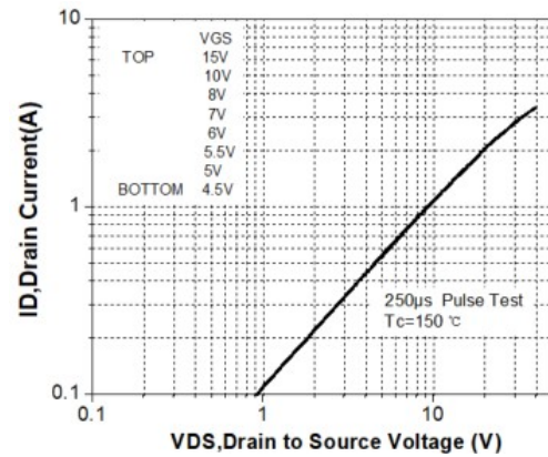
On-Region Characteristics
