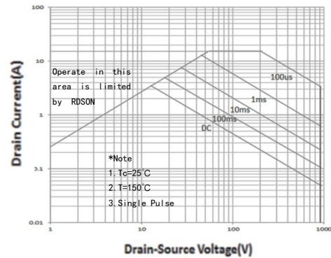
Maximum safe operating area for JCS4N95FA
