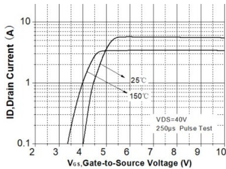
Transfer Characteristics
