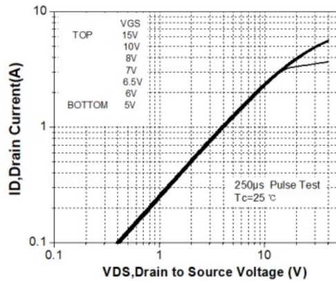
On-Region Characteristics
