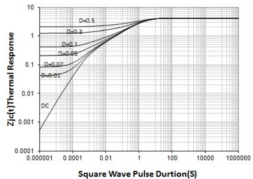
Transient Thermal Response Curve for JCS4N95FA
