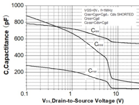
Capacitance Characteristics
