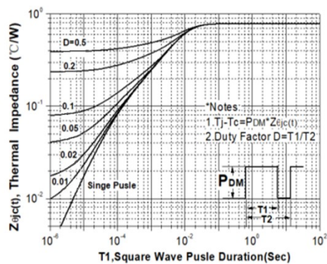
Transient Thermal Response Curve for JCS4N95RA/VA/CA/SA
