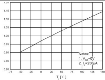
Breakdown Voltage Variation vs. Temperature
