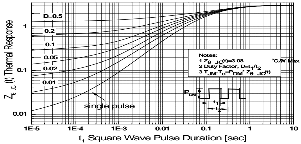
Transient Thermal Response Curve For JCS5N50FC
