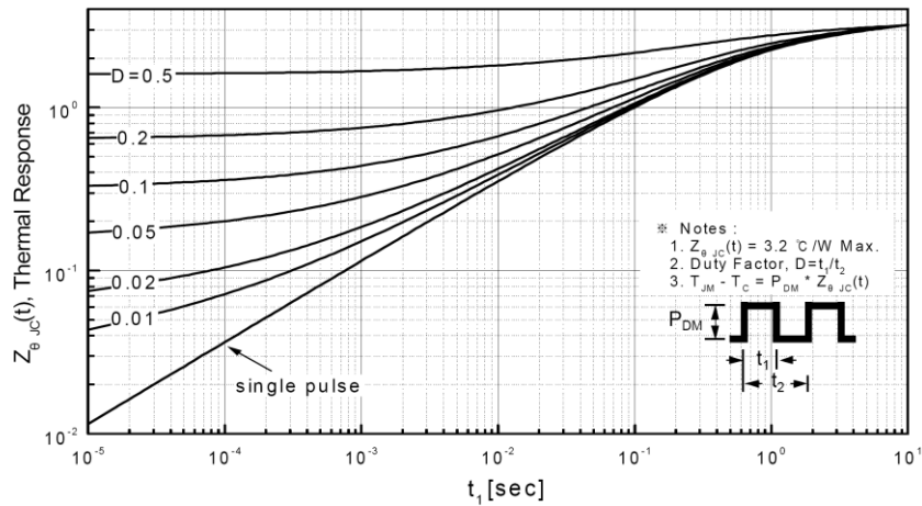
Transient Thermal Response Curve For JCS7HN60FC
