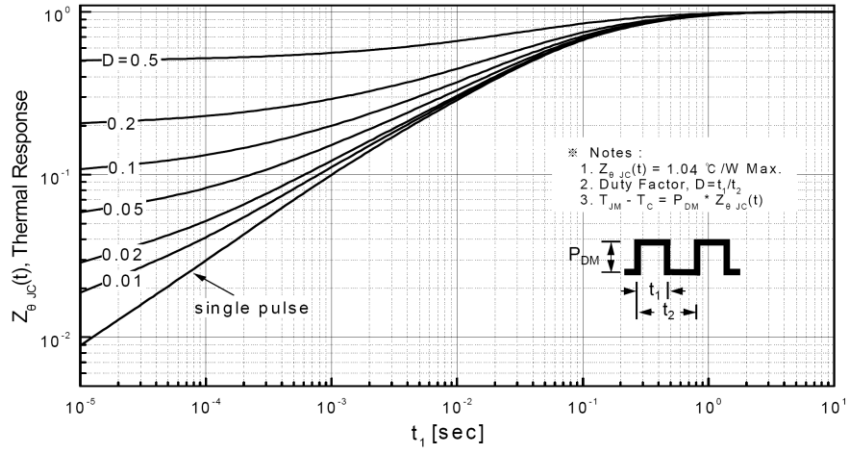
Transient Thermal Response Curve For JCS7HN60FC
