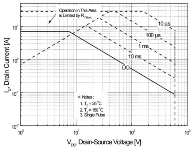
Maximum Safe Operating Area For JCS7HN60FC
