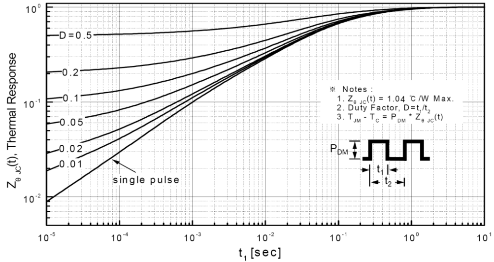
Transient Thermal Response Curve For JCS7N60CE/SE/BE/RE/VE
