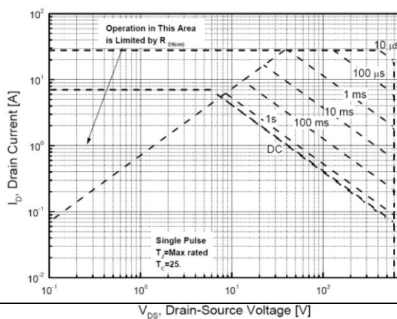
Maximum Safe Operating Area For JCS7N60CE/SE/BE/RE/VE
