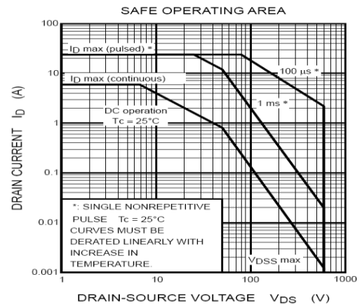
Maximum Safe Operating Area For JCS7N60FE
