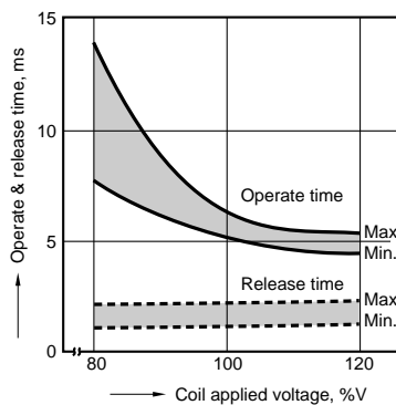
2. Operate and release time
