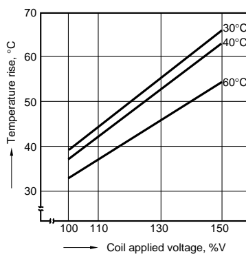
4. Coil temperature rise (Contact carrying current: 5 A)
