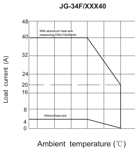
Figure 3 Maximum load current vs. ambient temperature
