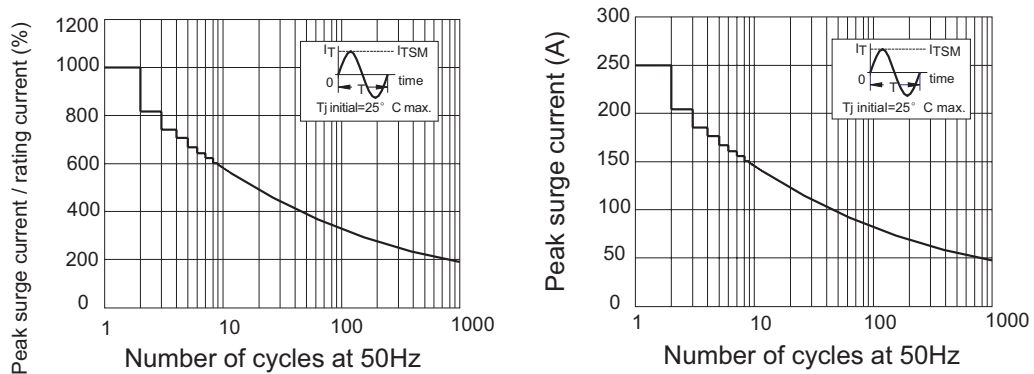
Figure 2 Maximum permissible non-repetitive peak surge current vs. Number of cycles
