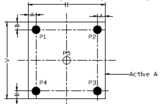
FIG.2. Measuring method for Contrast ratio, surface luminance, Luminance uniformity, CIE (x, y) chromaticity
