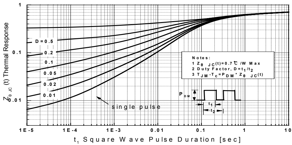
Transient Thermal Response Curve For JHW10N60CT
