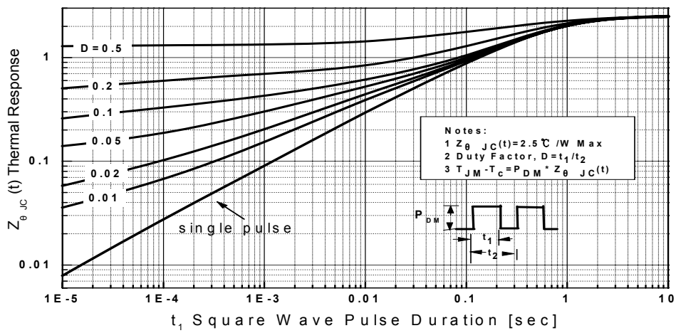
Transient Thermal Response Curve For JHW10N60FT
