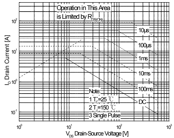
Maximum Safe Operating Area For JHW10N60FT
