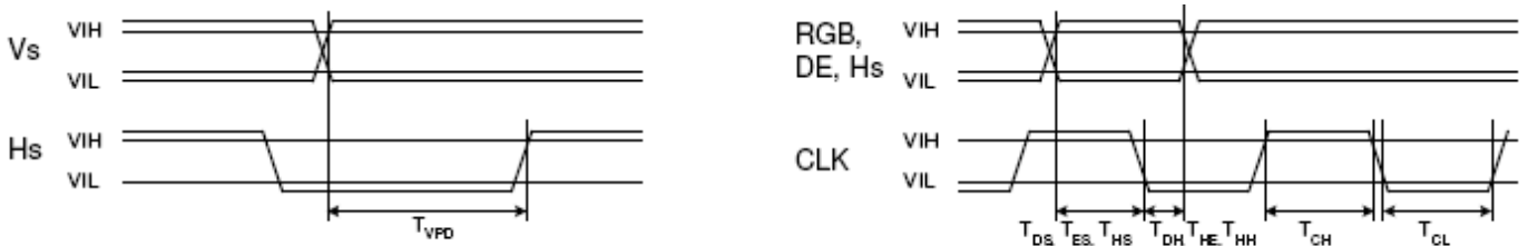
Figure 1 : Input timing details
