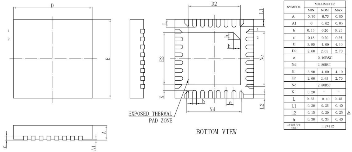
Figure 4-1 JL7016C Package
